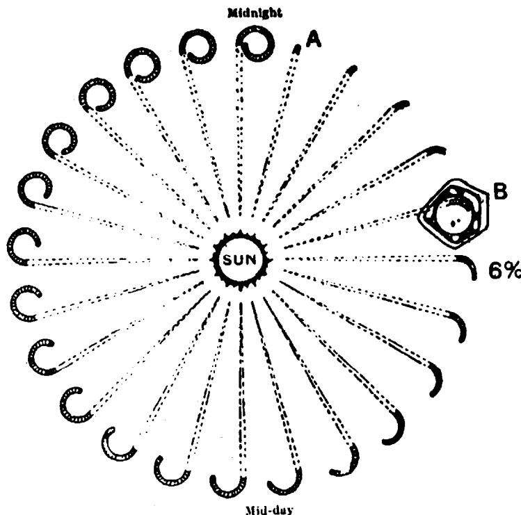
FIG. 22. FORMATION OF PRIMORDIAL CELL
