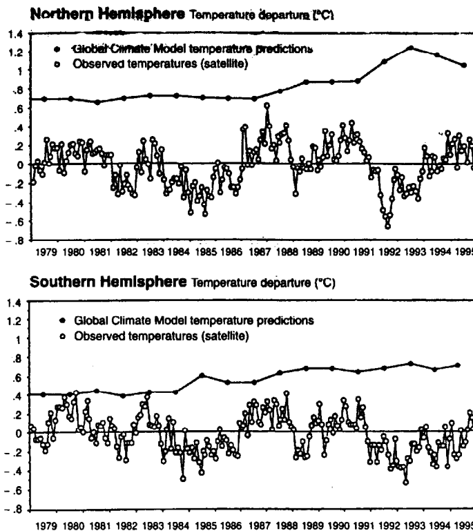
FIGURE 1 Climate Model Predictions vs. Satellite Measurements
